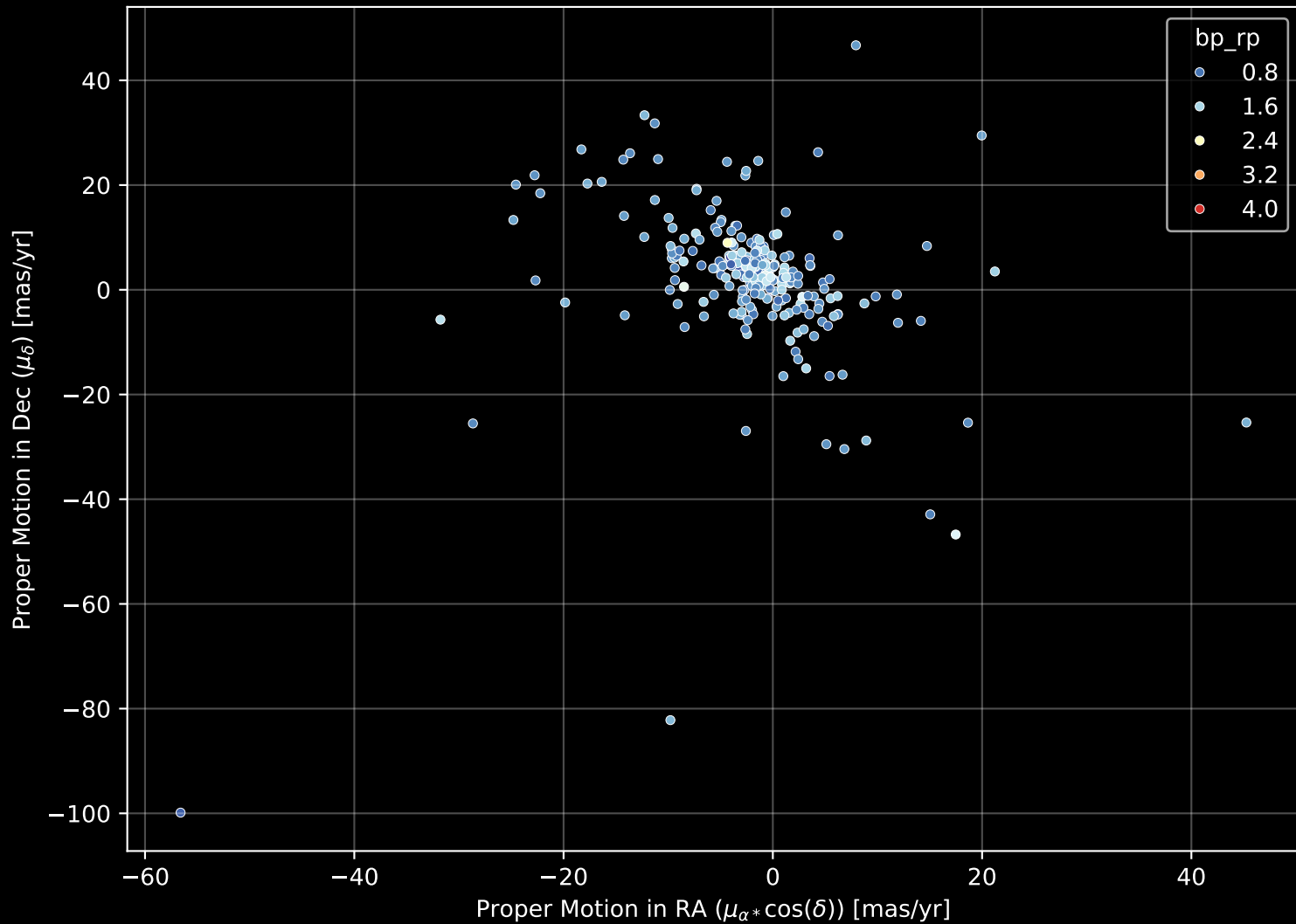
GALAH DR4 Field: [3545] Proper Motion Diagram (n= 263)
