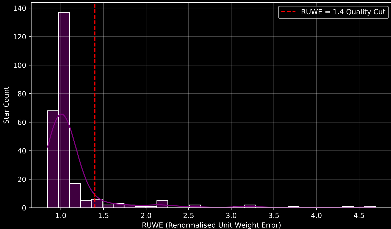
GALAH DR4 Field [3545] RUWE Distribution (n= 255)
