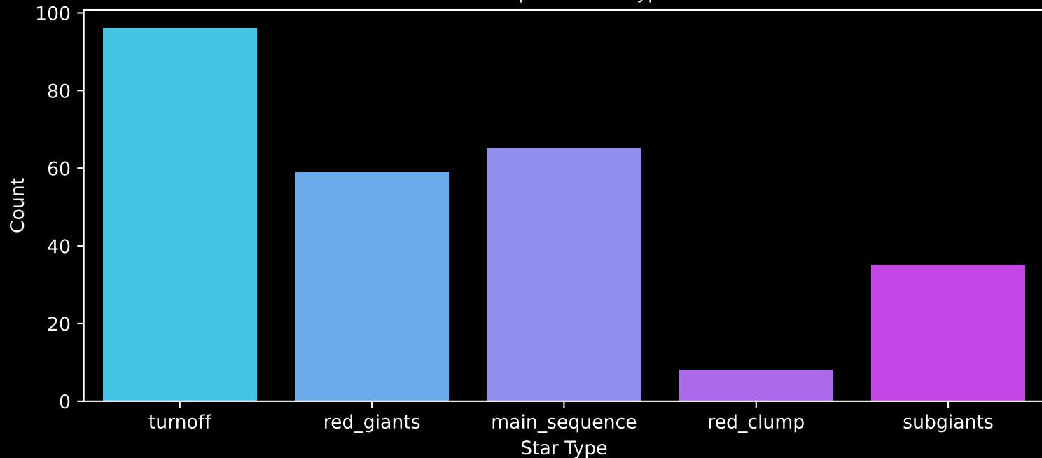
GALAH DR4 Field: [3545] Count plot of Star Type
